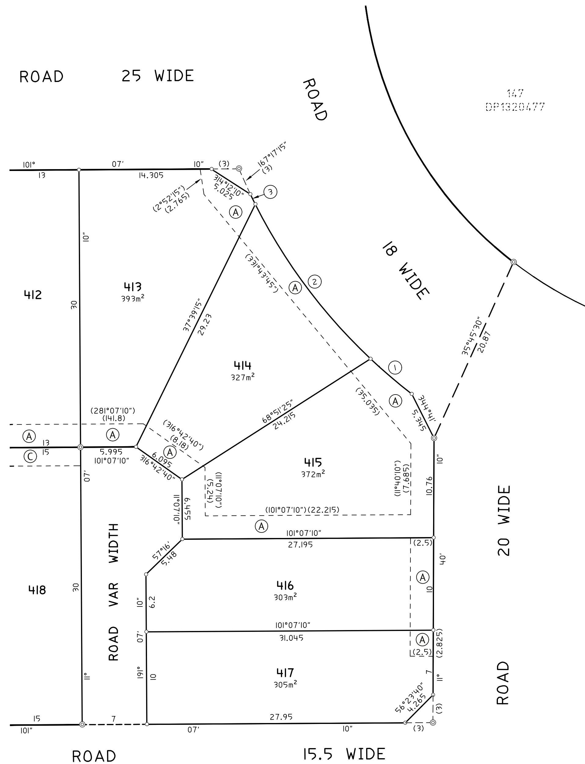
DIAGRAM SCALE 1:250
